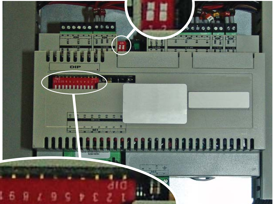
Dip-switch (B)
